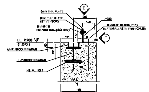
SEC. N-N (C 1) SC 120
