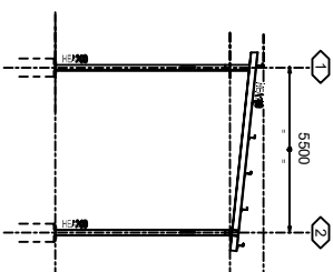
FRAME ON AXIS B SC: 1100
