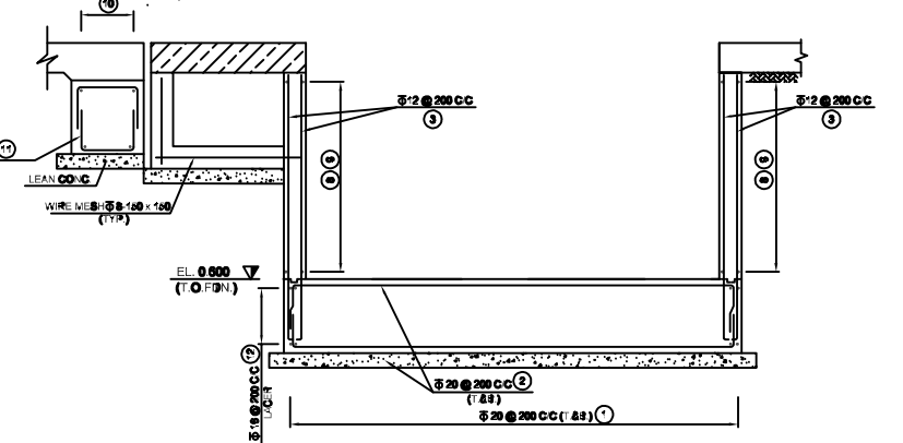
SEC. I-I (C 1) SC 120
