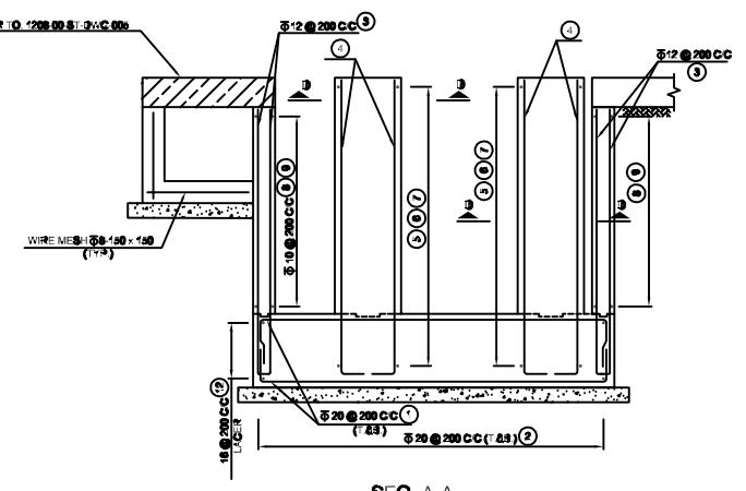
SEC. A-A (C 1) SC 120
