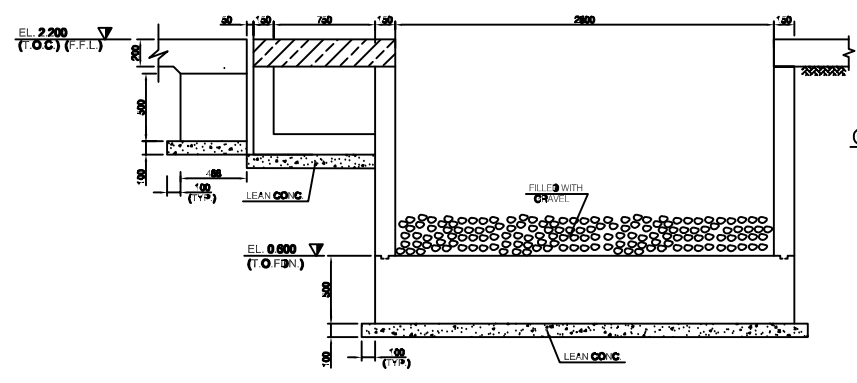
SEC. I-I (C 1) SC 120
