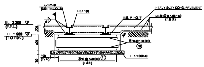
SEC. C-C (C 1) SC 120
