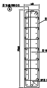
SEC. D-D (C 1) SC 120
