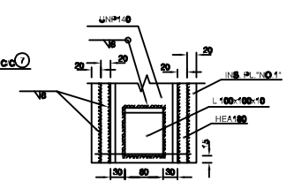
DET. "1" (C 1) SC 120
