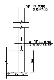
VIEW "B" (C 1) SC 120
