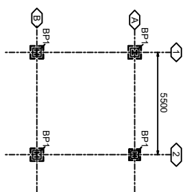
PLANAT (B.O.BASE.P.L.)
