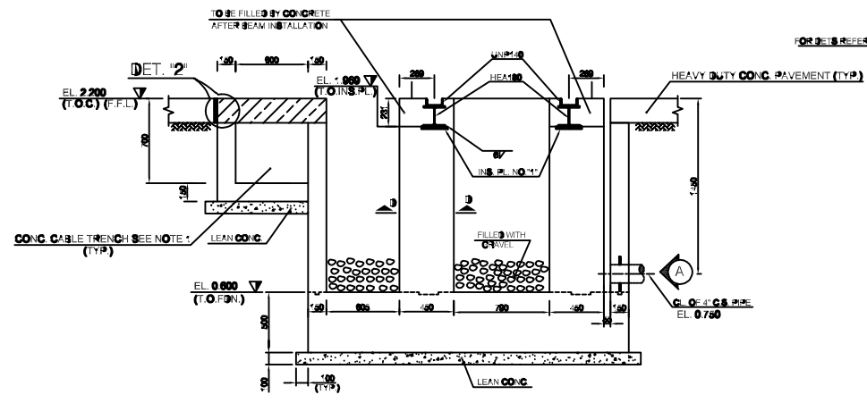
SEC. A-A (C 1) SC 120
