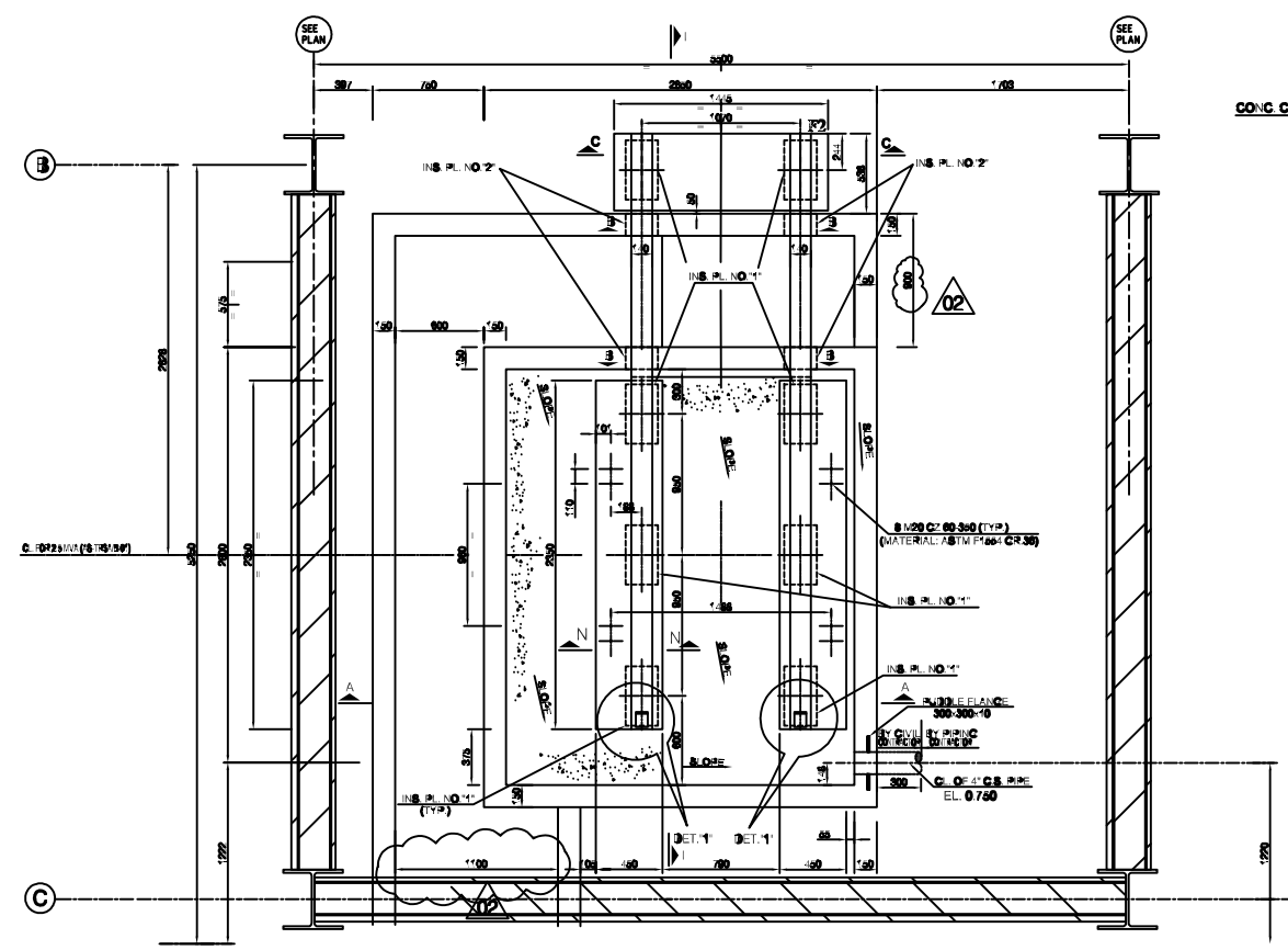
FDN. "F1" & "F2" (4X) (C 1) SC 120
